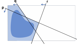
Fig. 2. Example space where ite(p, r, q \wedge r) < r .
