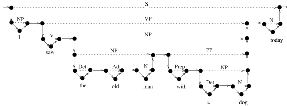
FIG. 4. Parsed sentence as a nested word.
