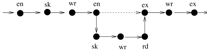
FIG. 3. Sample program execution.
