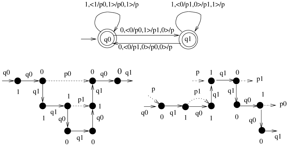
FIG. 6. Example of an NWA and its runs.
