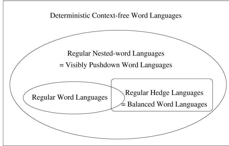
FIG. 12. Relationship among languages classes.
