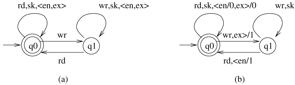
FIG. 7. Program requirements as NWAs.
